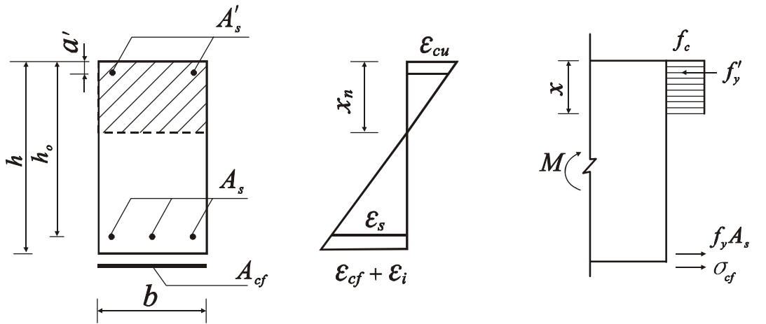
(a) x > \xi_{cfb}h 时
